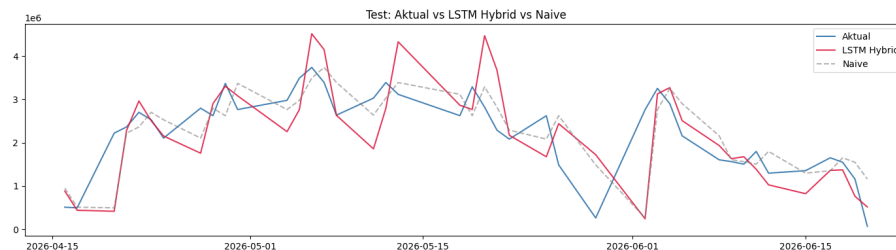
Figure 2. Time Series Comparison of Actual Canteen Revenue Against Hybrid LSTM Model Forecasts
